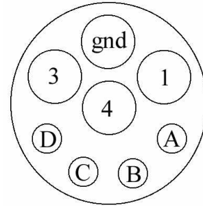
Type 8 Connector seen from motor outside
