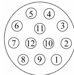
Type 12 Connector seen from motor outside
